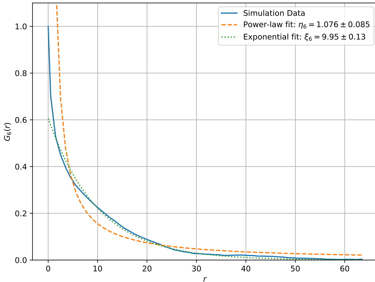
Correlation Function at T = 2.00e - 01 , L = 128
