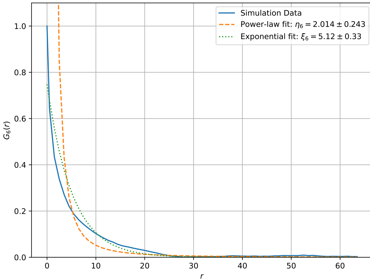
Correlation Function at T = 2.10e - 01, L = 128
