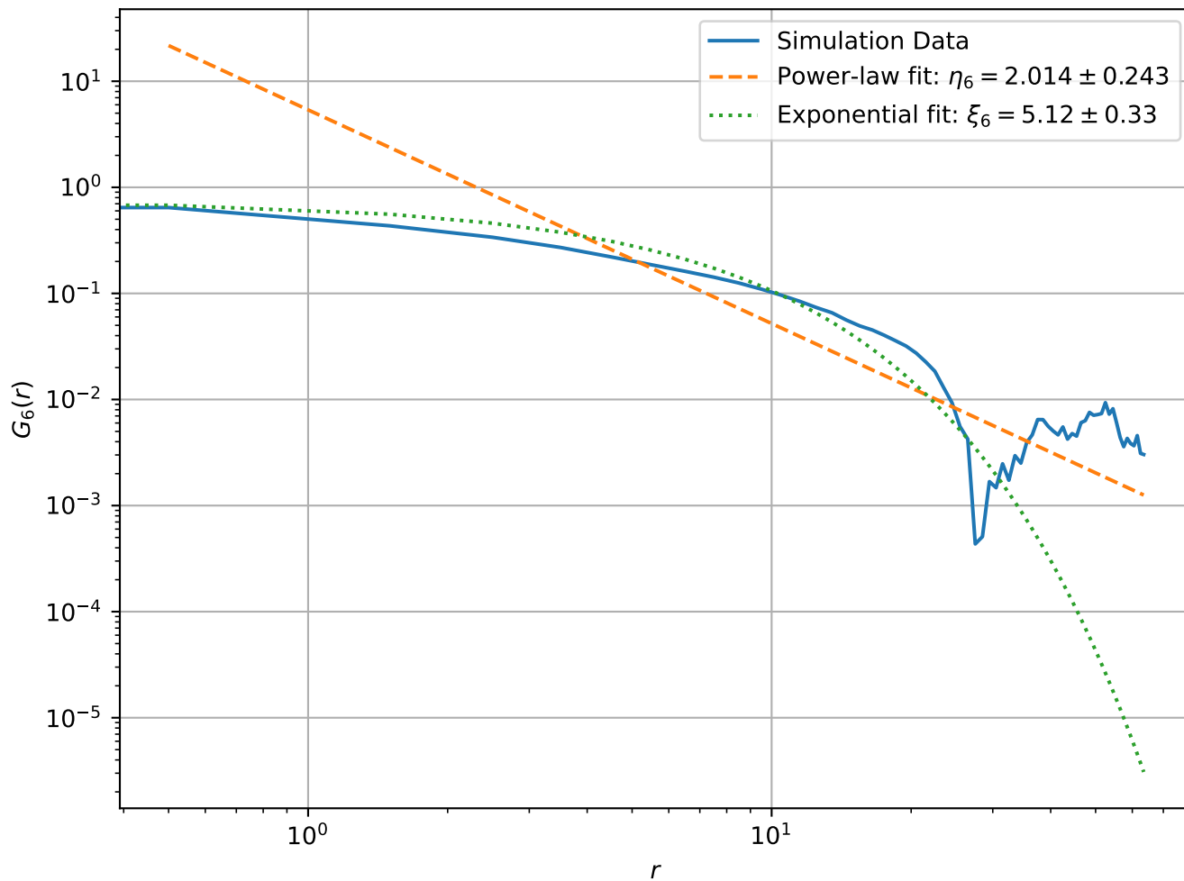
Correlation Function at T = 2.10e - 01 , L = 128 (Log-Log Scale)
