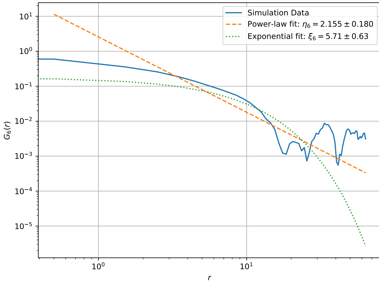
Correlation Function at T = 2.20e - 01 , L = 128 (Log-Log Scale)
