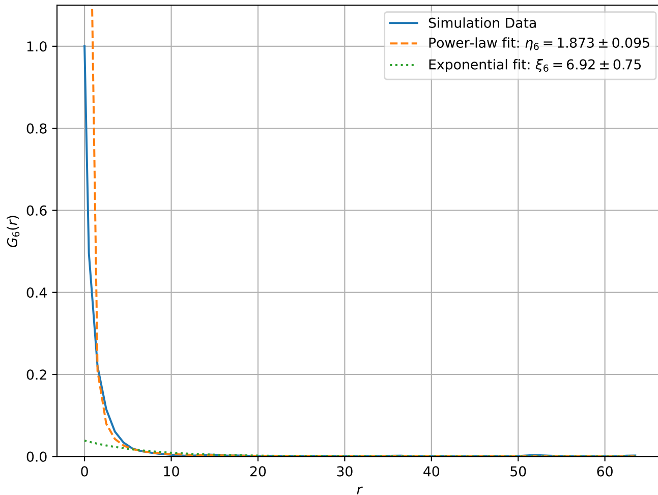
Correlation Function at T = 2.50e - 01 , L = 128
