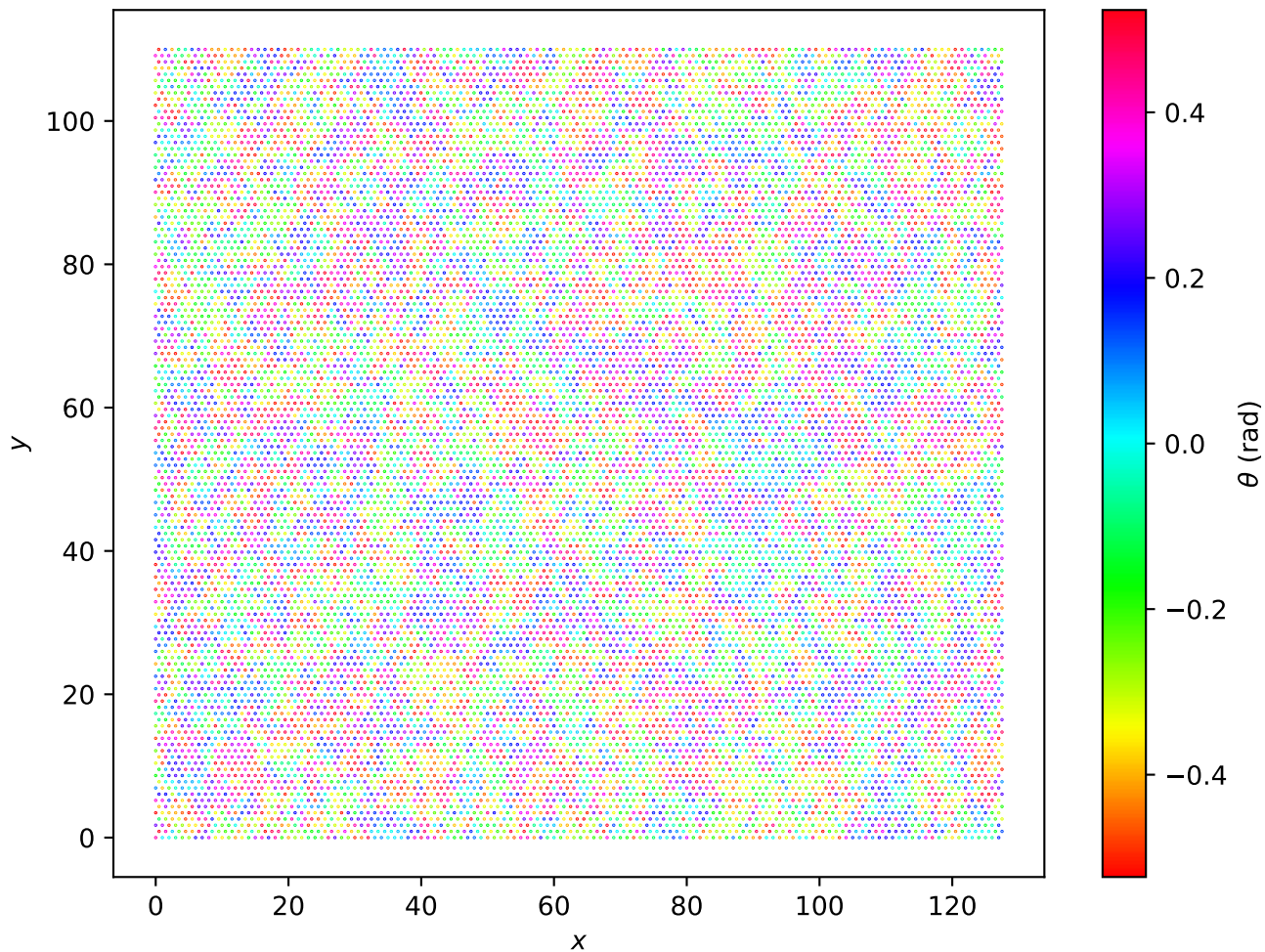
Hexagonal Lattice L=128 , T = 2.50e - 01
