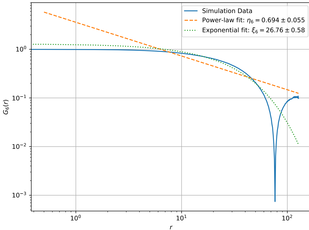
Correlation Function at T = 1.00e - 05 , L = 256 (Log-Log Scale)
