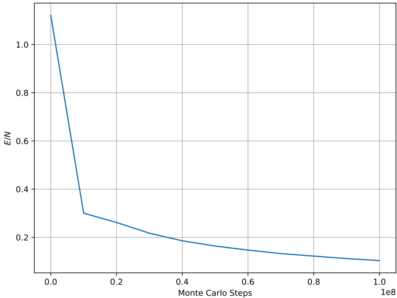
Energy per Spin at T = 1.00e - 05 , L = 256
