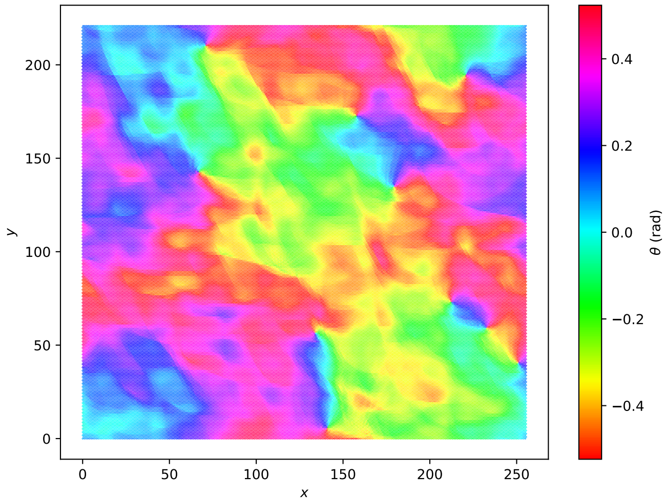
Hexagonal Lattice L=256 , T = 1.00e - 05
