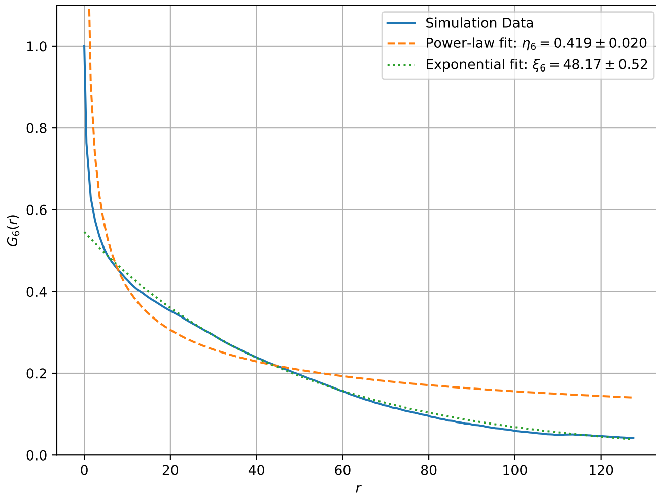
Correlation Function at T = 1.90e - 01, L = 256
