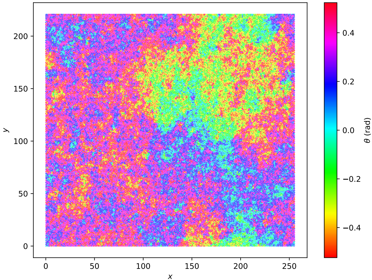
Hexagonal Lattice L=256 , T = 1.90e - 01
