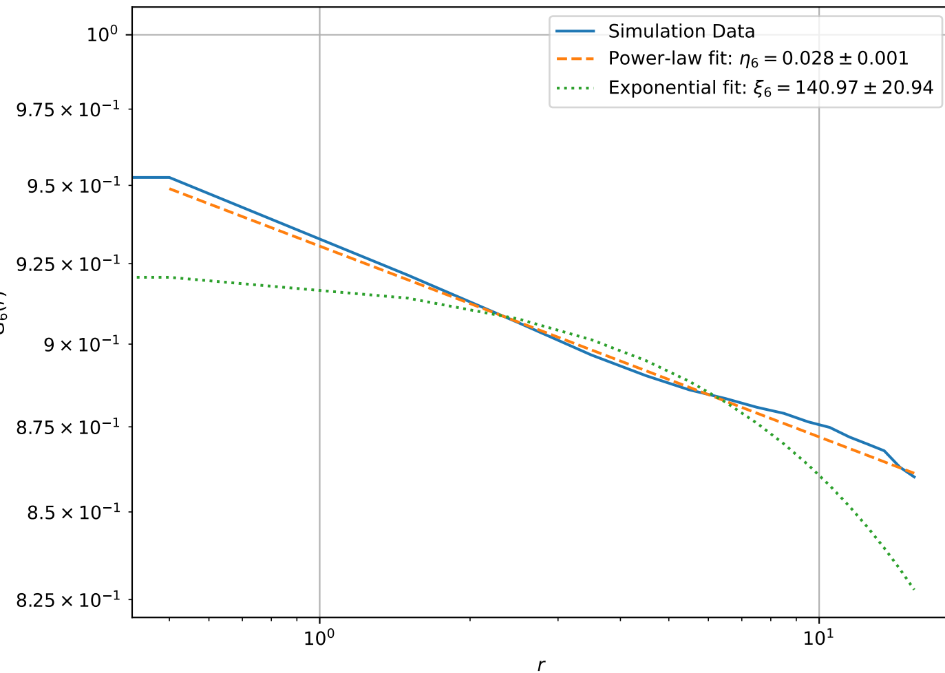
Correlation Function at T = 1.20e - 01 , L = 32 (Log-Log Scale)
