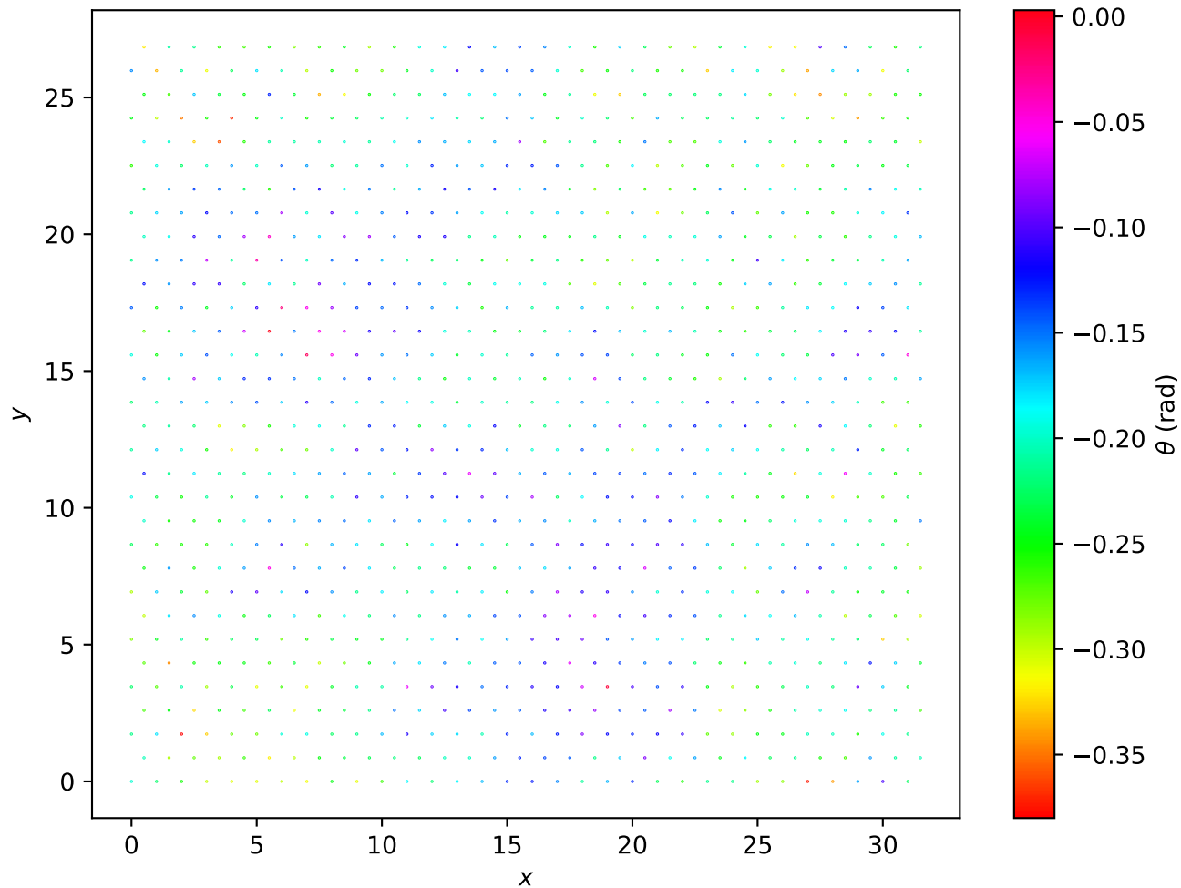
Hexagonal Lattice L=32 , T = 1.20e - 01
