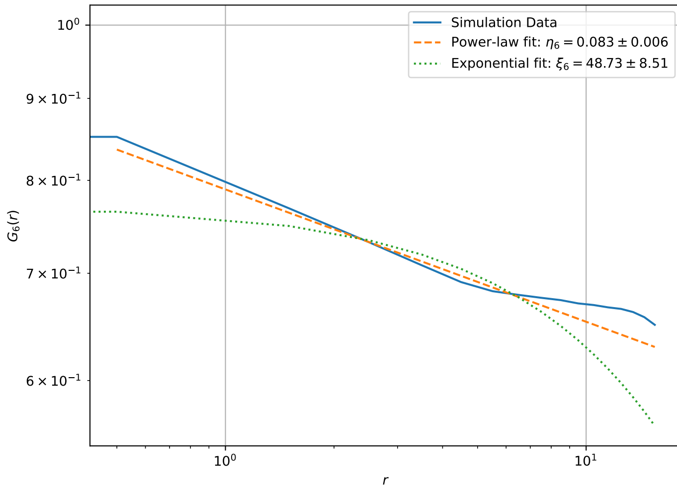
Correlation Function at T = 1.70e - 01 , L = 32 (Log-Log Scale)
