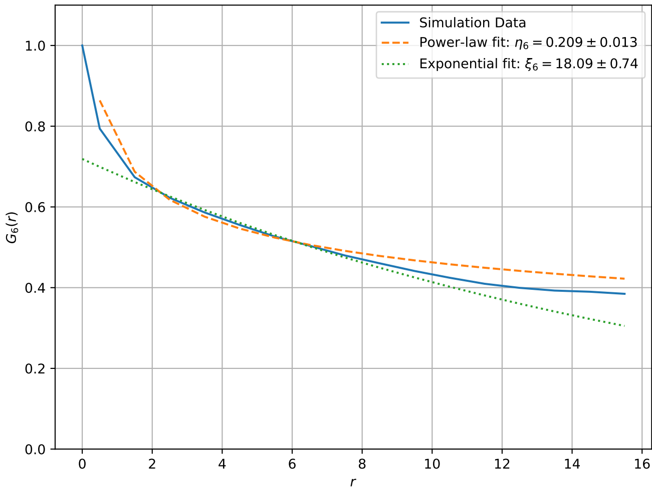
Correlation Function at T = 1.80e - 01 , L = 32
