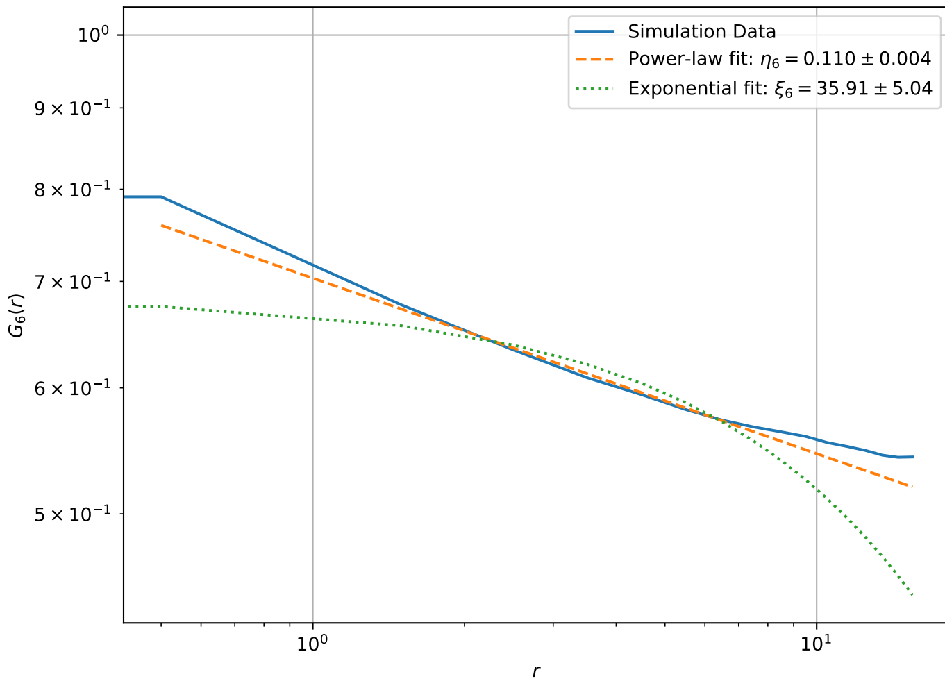
Correlation Function at T = 1.90e - 01 , L = 32 (Log-Log Scale)
