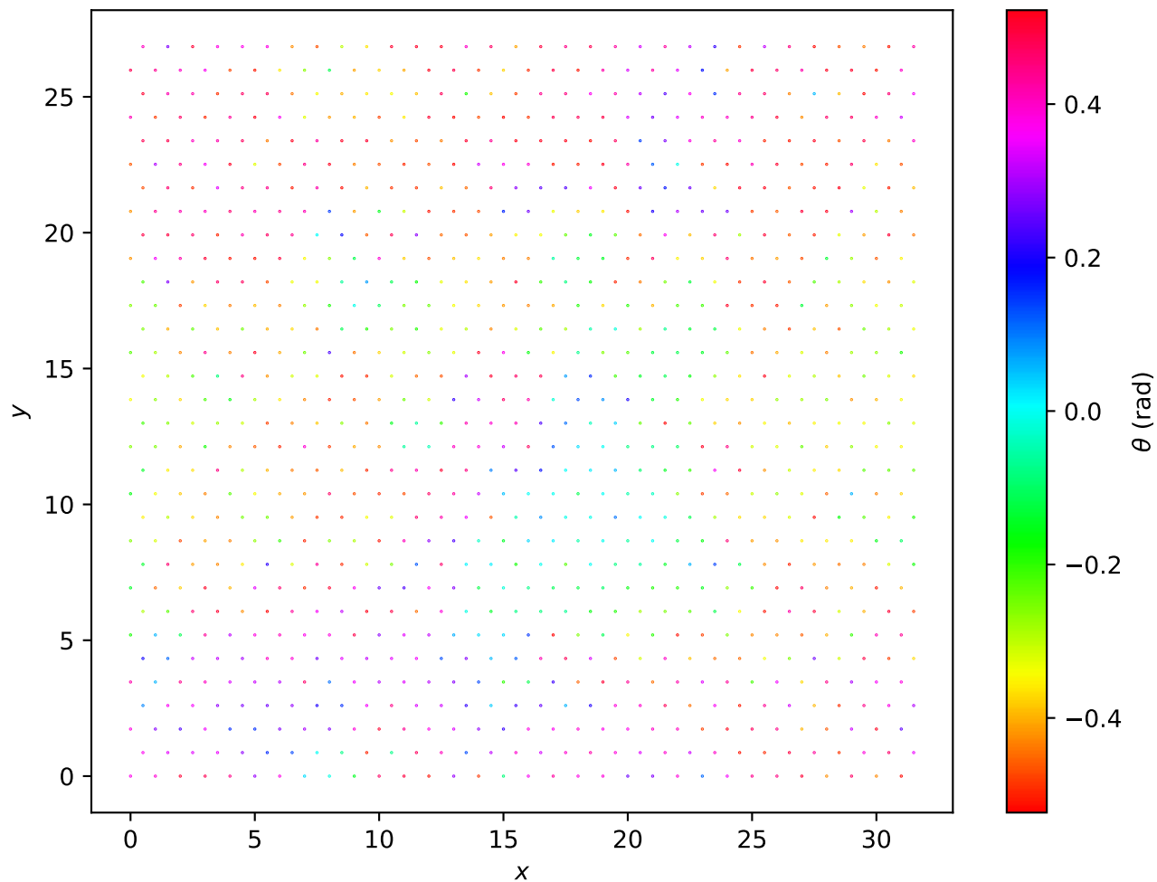
Hexagonal Lattice L=32 , T = 2.00e - 01
