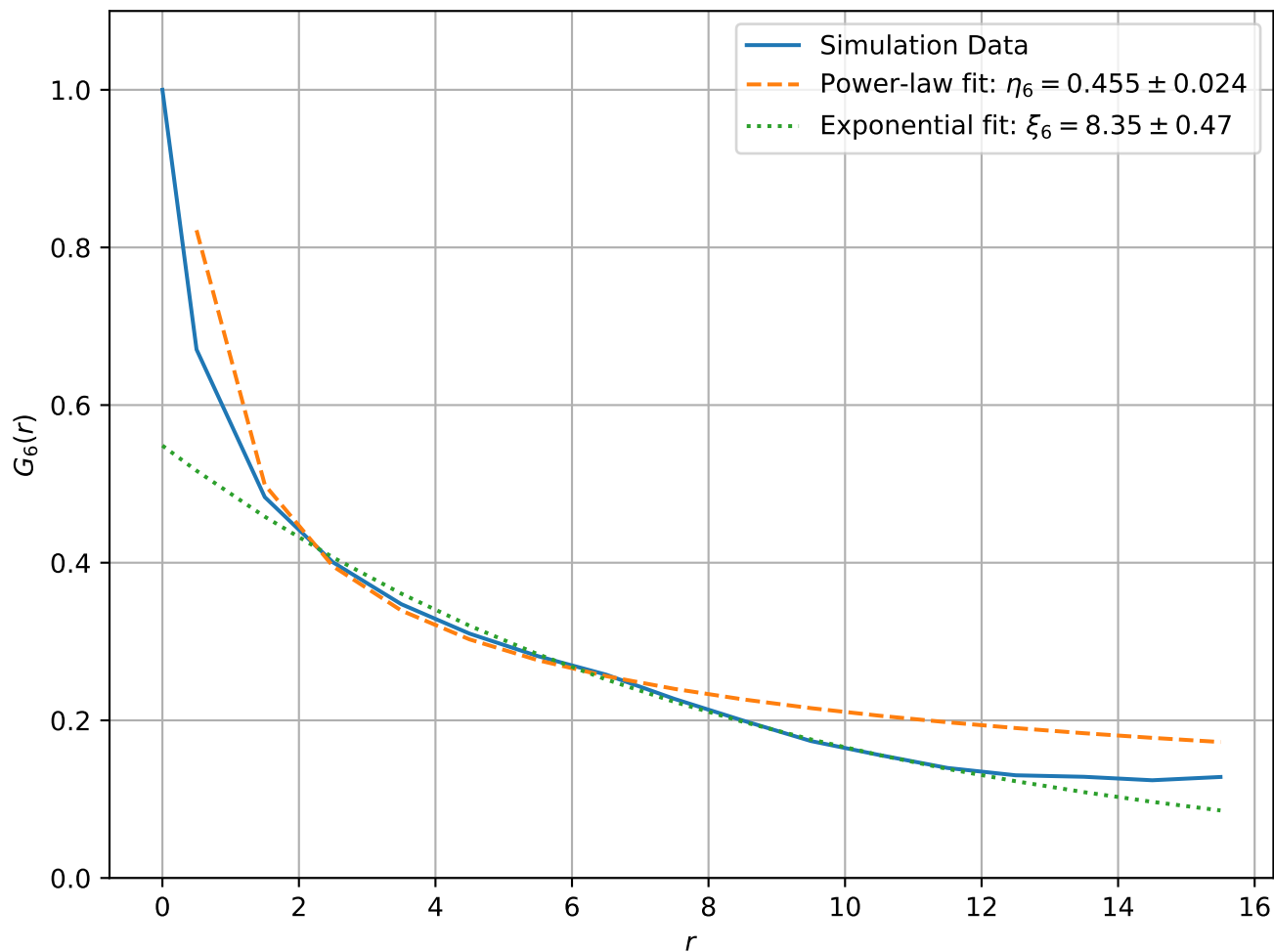
Correlation Function at T = 2.10e - 01 , L = 32
