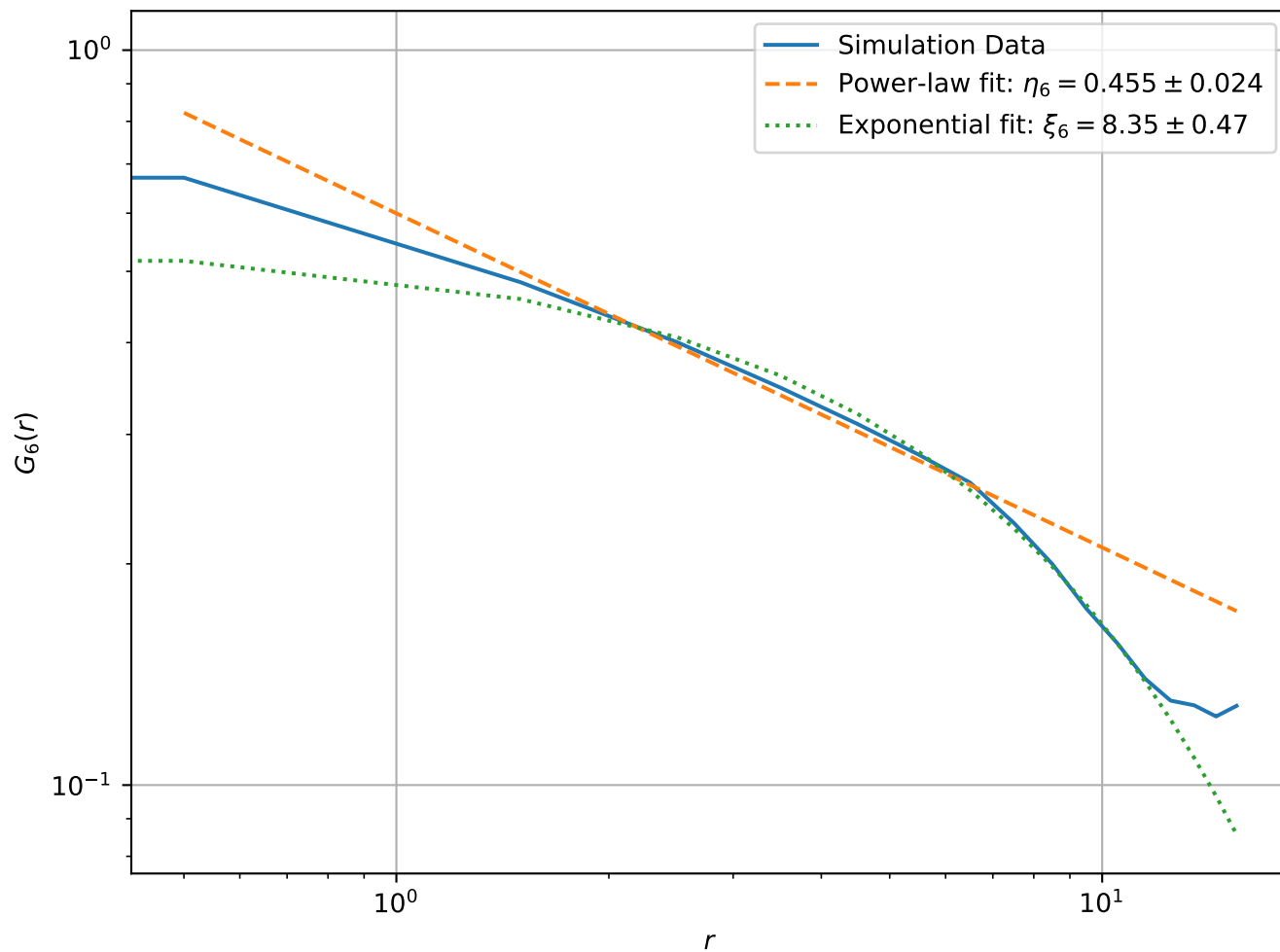
Correlation Function at T = 2.10e - 01 , L = 32 (Log-Log Scale)
