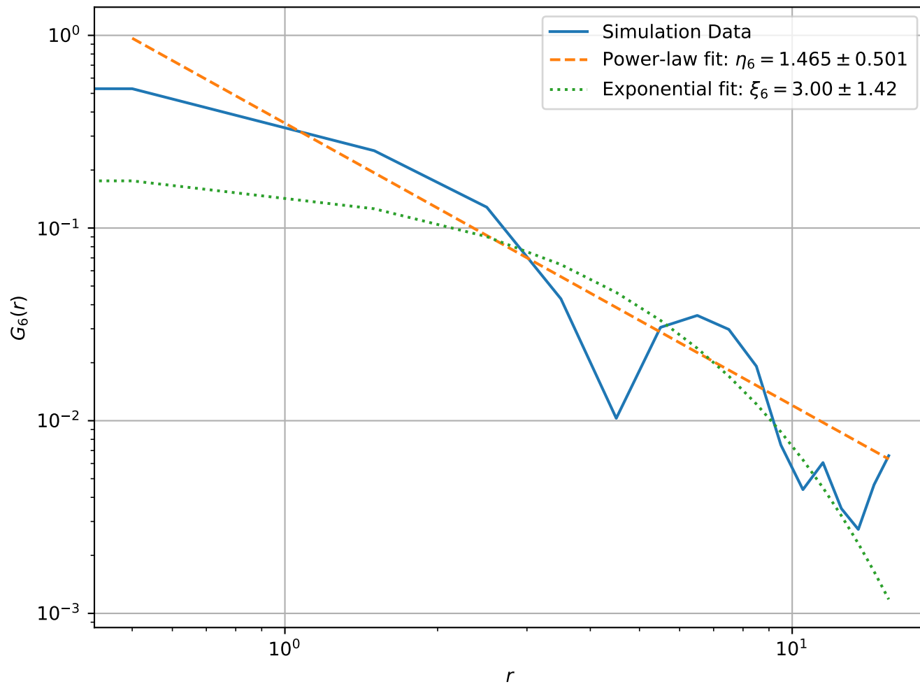
Correlation Function at T = 2.50e - 01 , L = 32 (Log-Log Scale)
