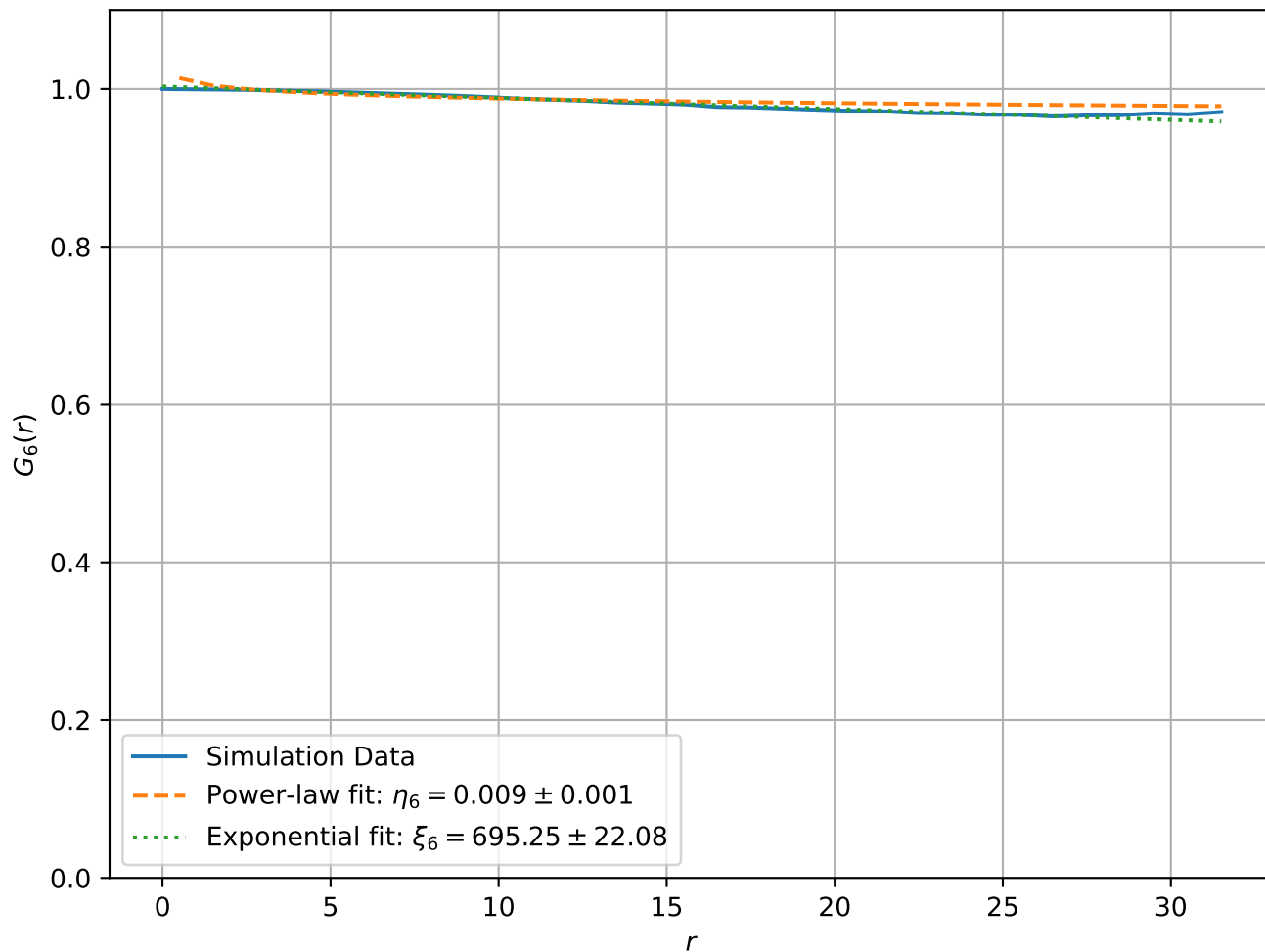
Correlation Function at T = 1.00e - 02 , L = 64
