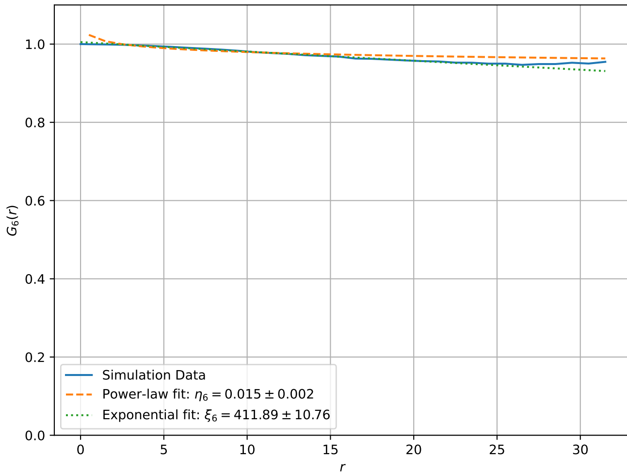
Correlation Function at T = 1.00e - 05 , L = 64
