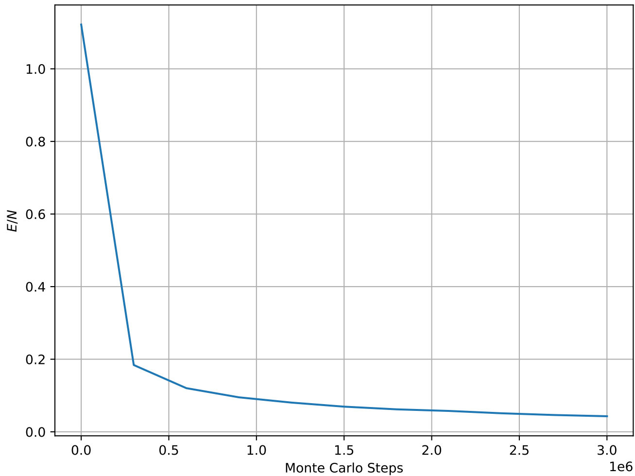
Energy per Spin at T = 1.00e - 05 , L = 64
