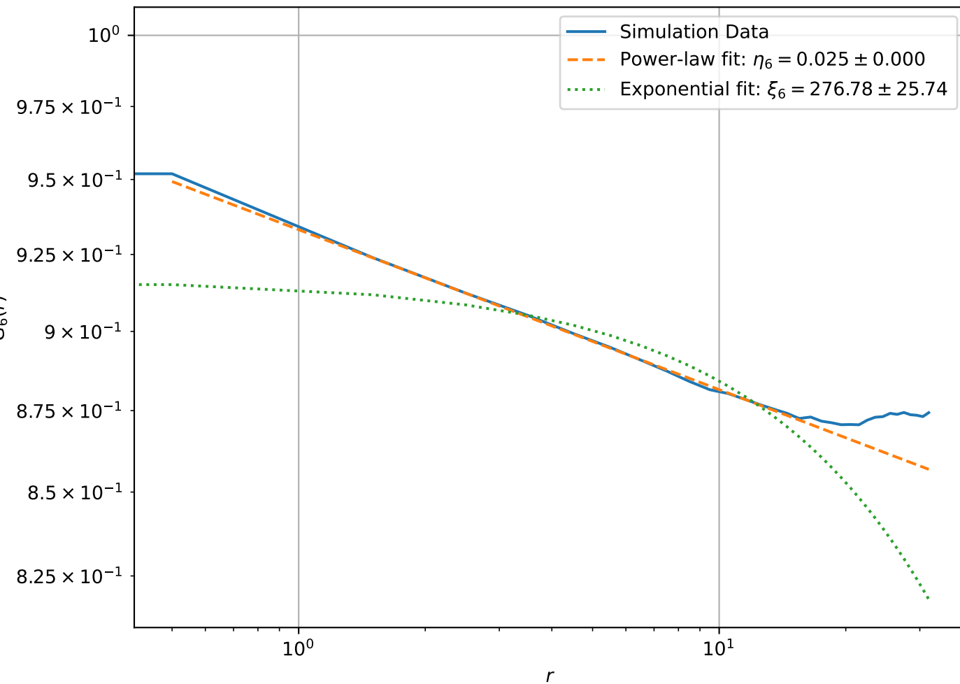
Correlation Function at T = 1.20e - 01 , L = 64 (Log-Log Scale)
