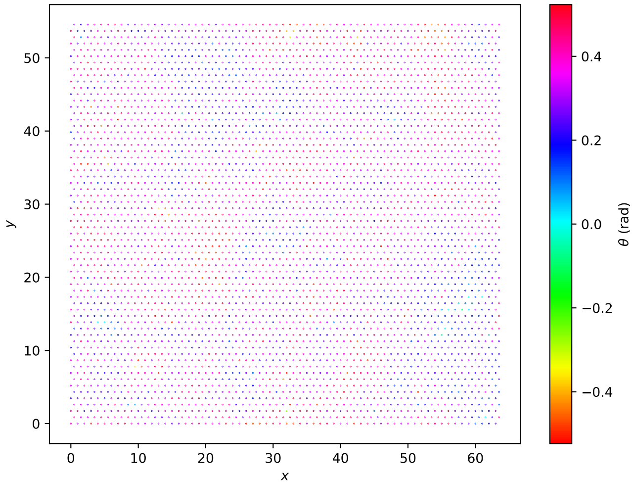
Hexagonal Lattice L=64 , T = 1.50e - 01
