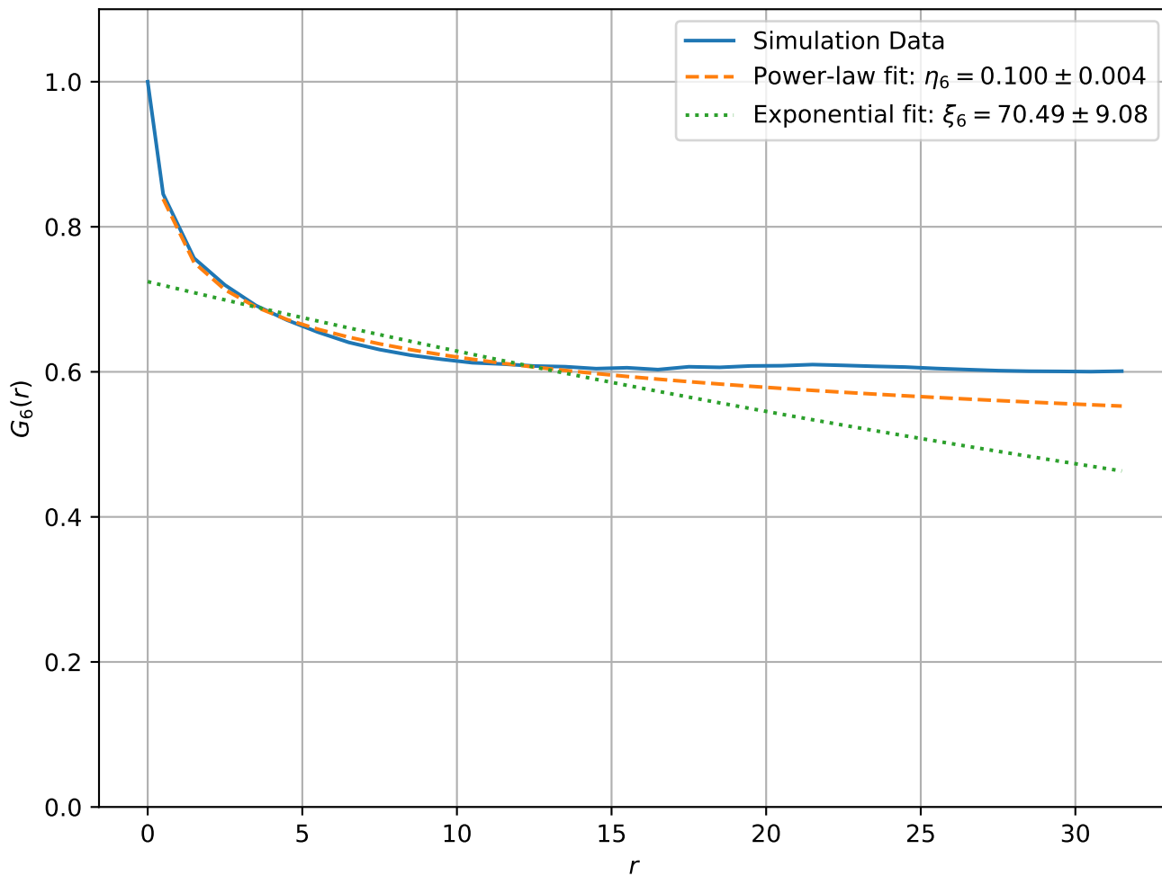
Correlation Function at T = 1.70e - 01 , L = 64
