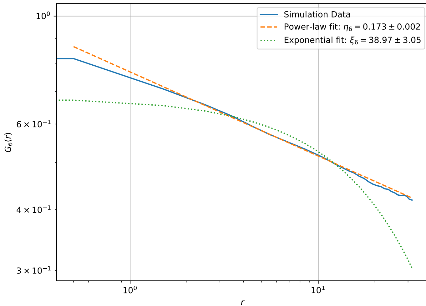
Correlation Function at T = 1.80e - 01 , L = 64 (Log-Log Scale)
