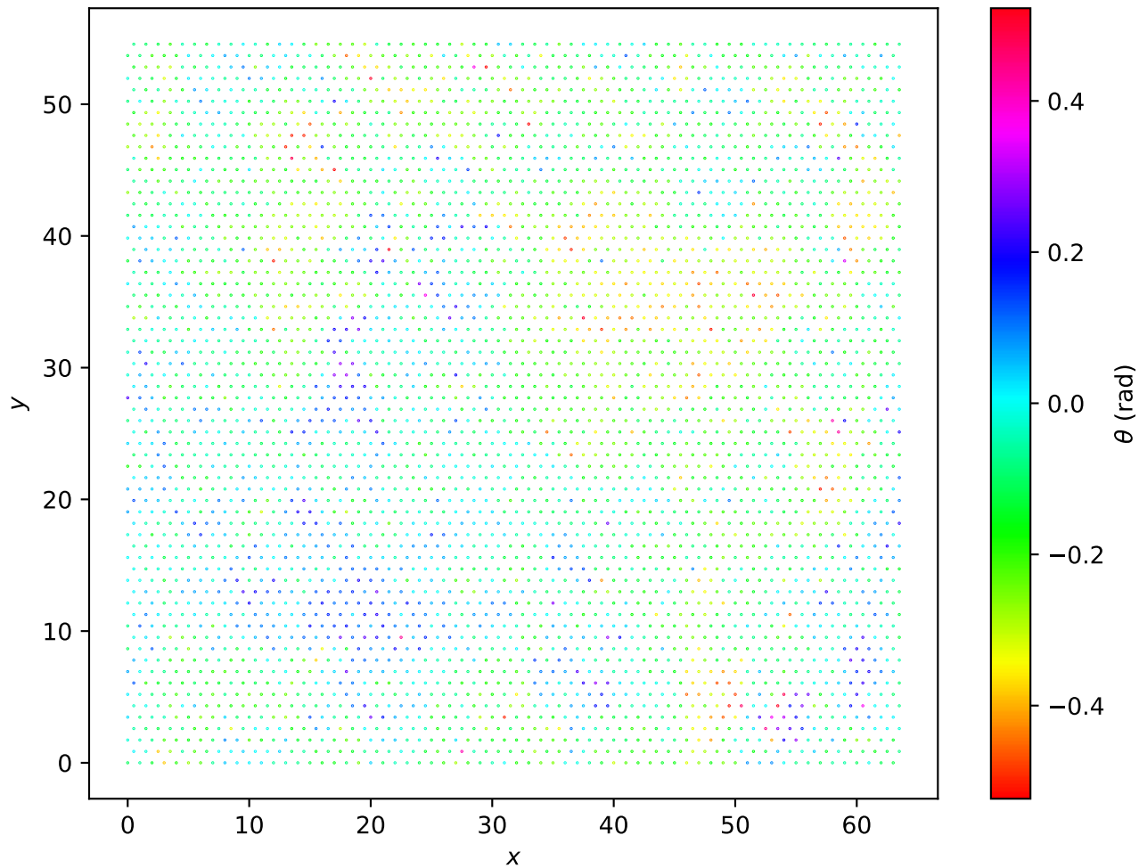
Hexagonal Lattice L=64 , T = 1.80e - 01
