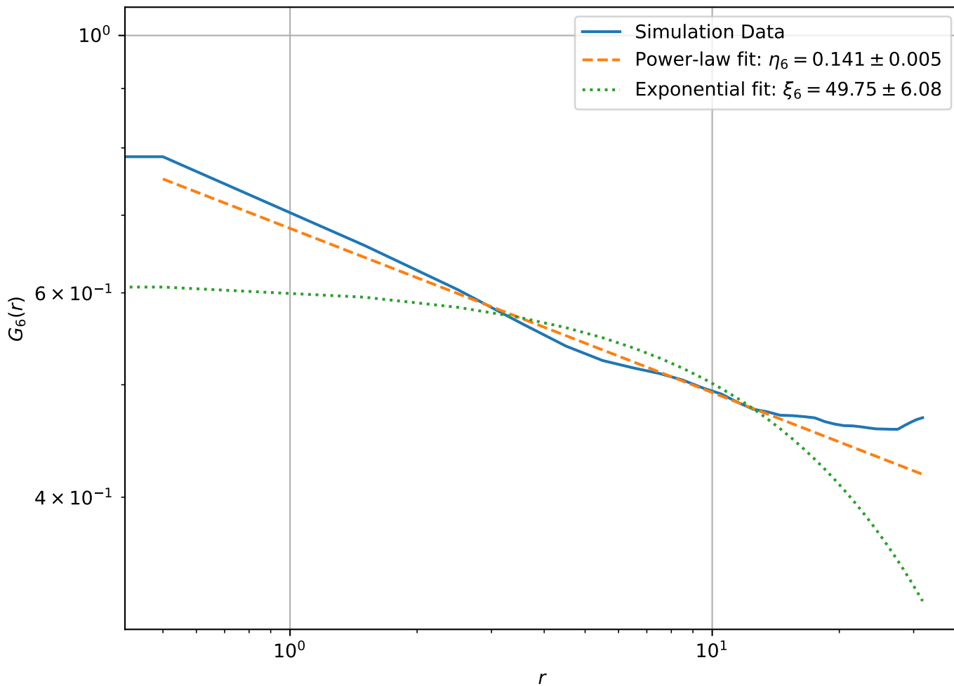
Correlation Function at T = 1.90e - 01 , L = 64 (Log-Log Scale)
