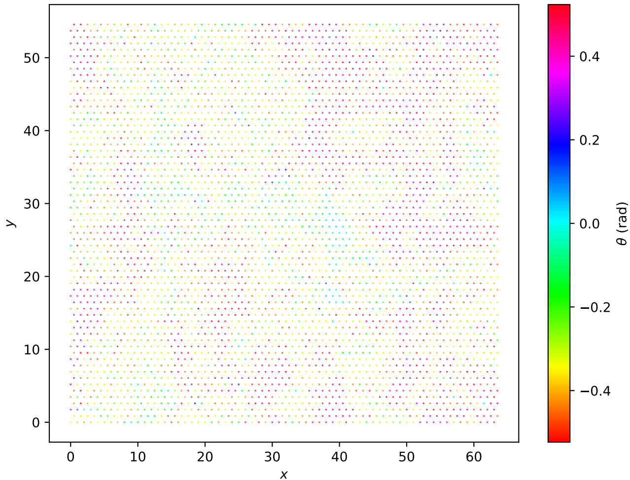
Hexagonal Lattice L=64 , T = 1.90e - 01
