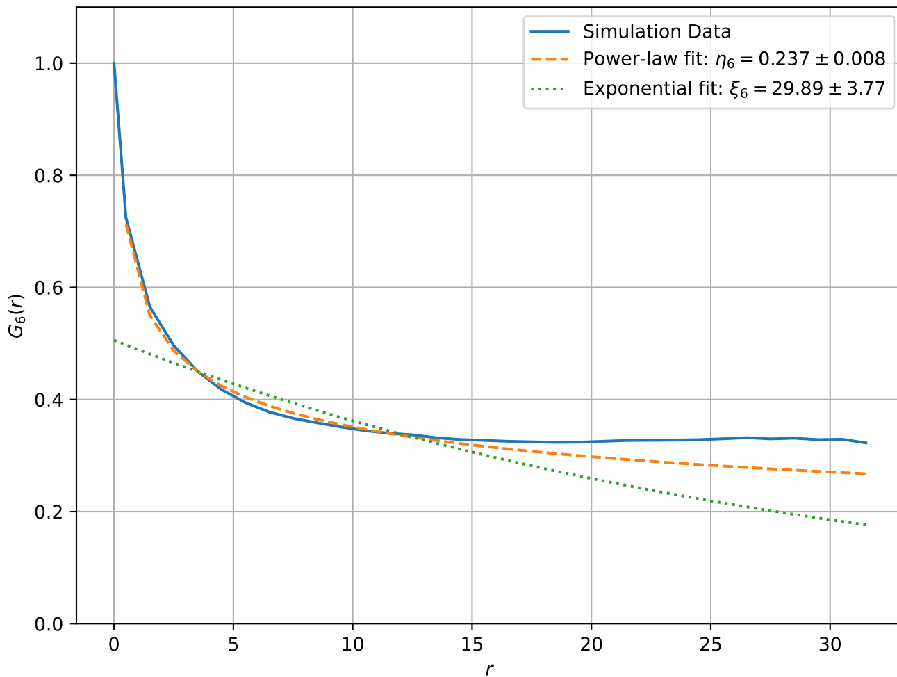
Correlation Function at T = 2.00e - 01 , L = 64
