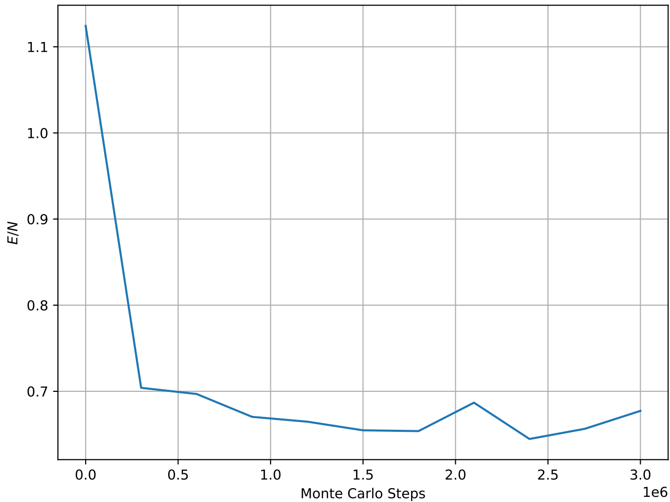
Energy per Spin at T = 2.00e - 01 , L = 64
