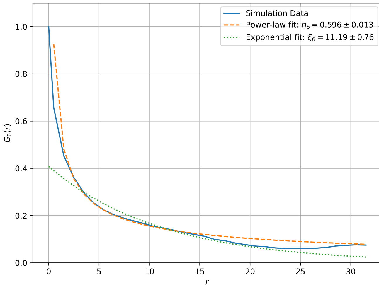
Correlation Function at T = 2.10e - 01 , L = 64
