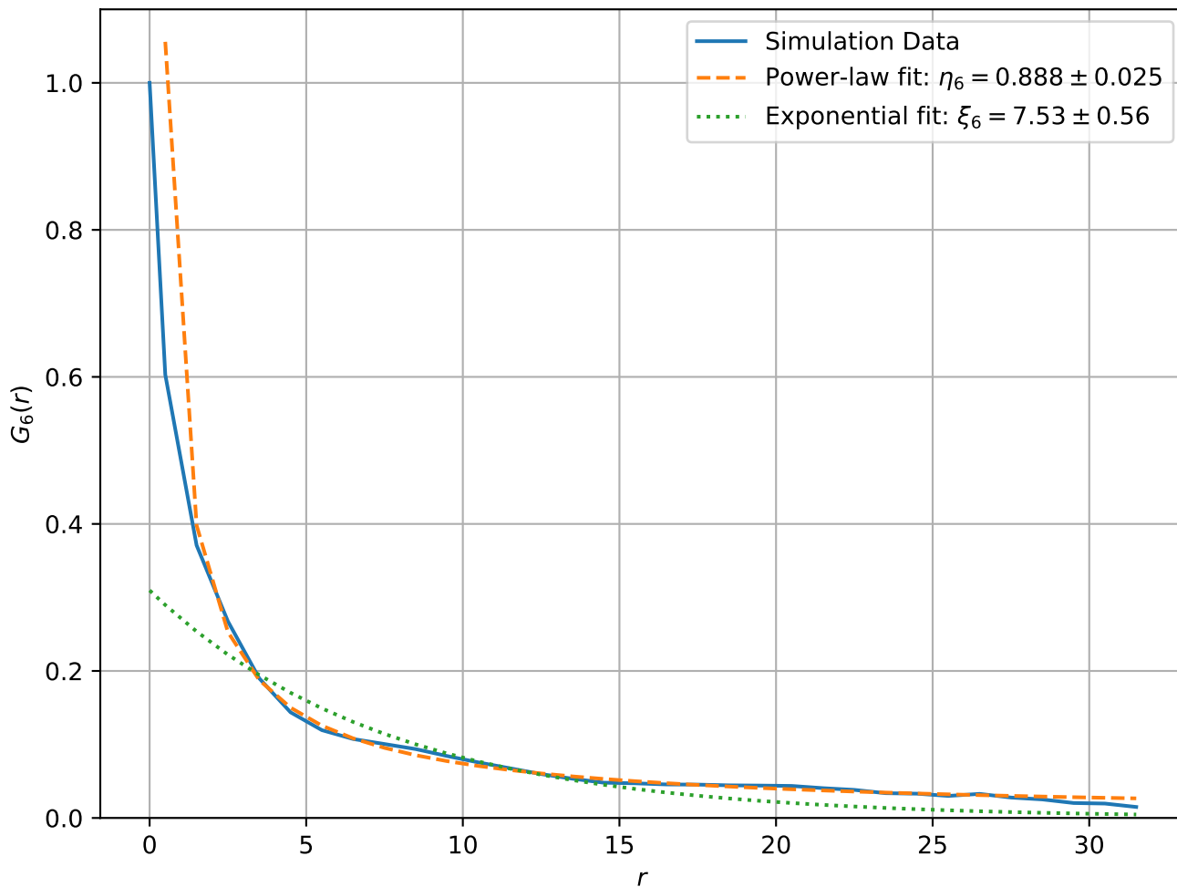
Correlation Function at T = 2.20e - 01 , L = 64
