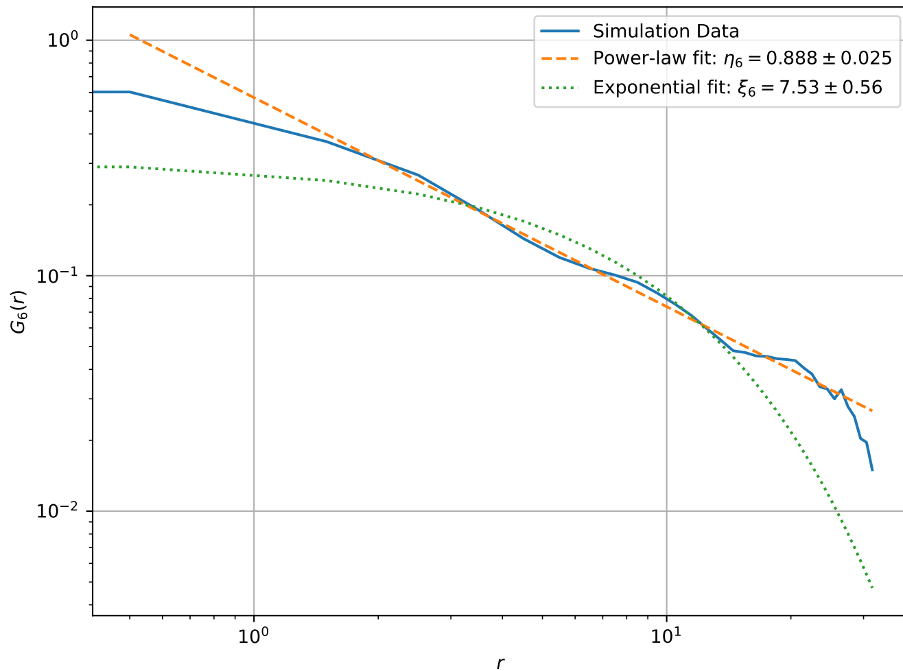
Correlation Function at T = 2.20e - 01 , L = 64 (Log-Log Scale)
