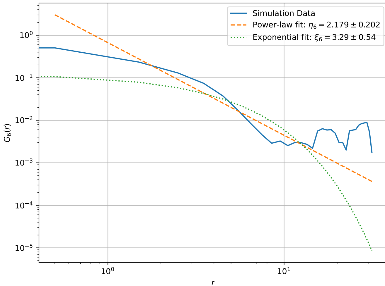
Correlation Function at T = 2.50e - 01 , L = 64 (Log-Log Scale)
