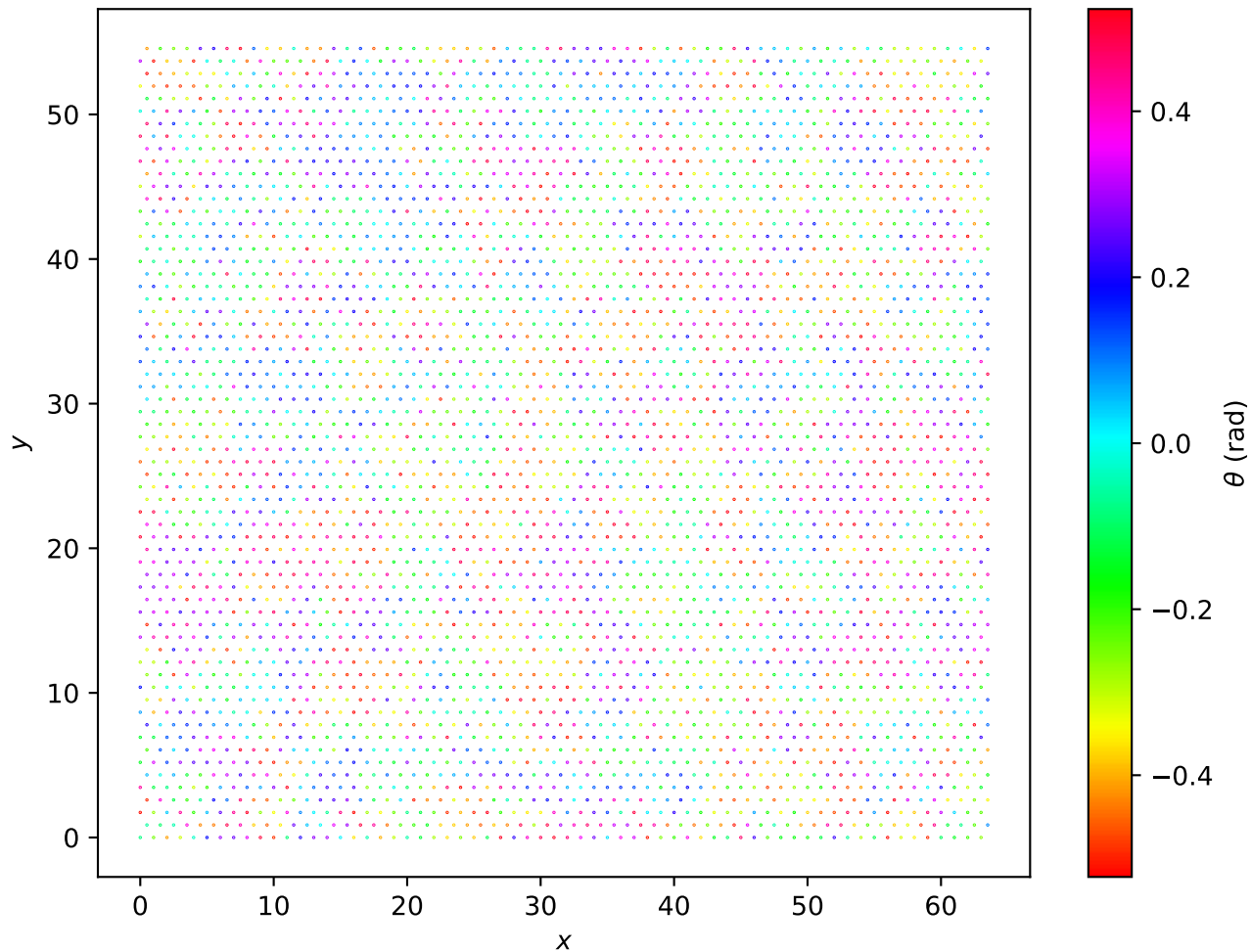
Hexagonal Lattice L=64 , T = 2.50e - 01
