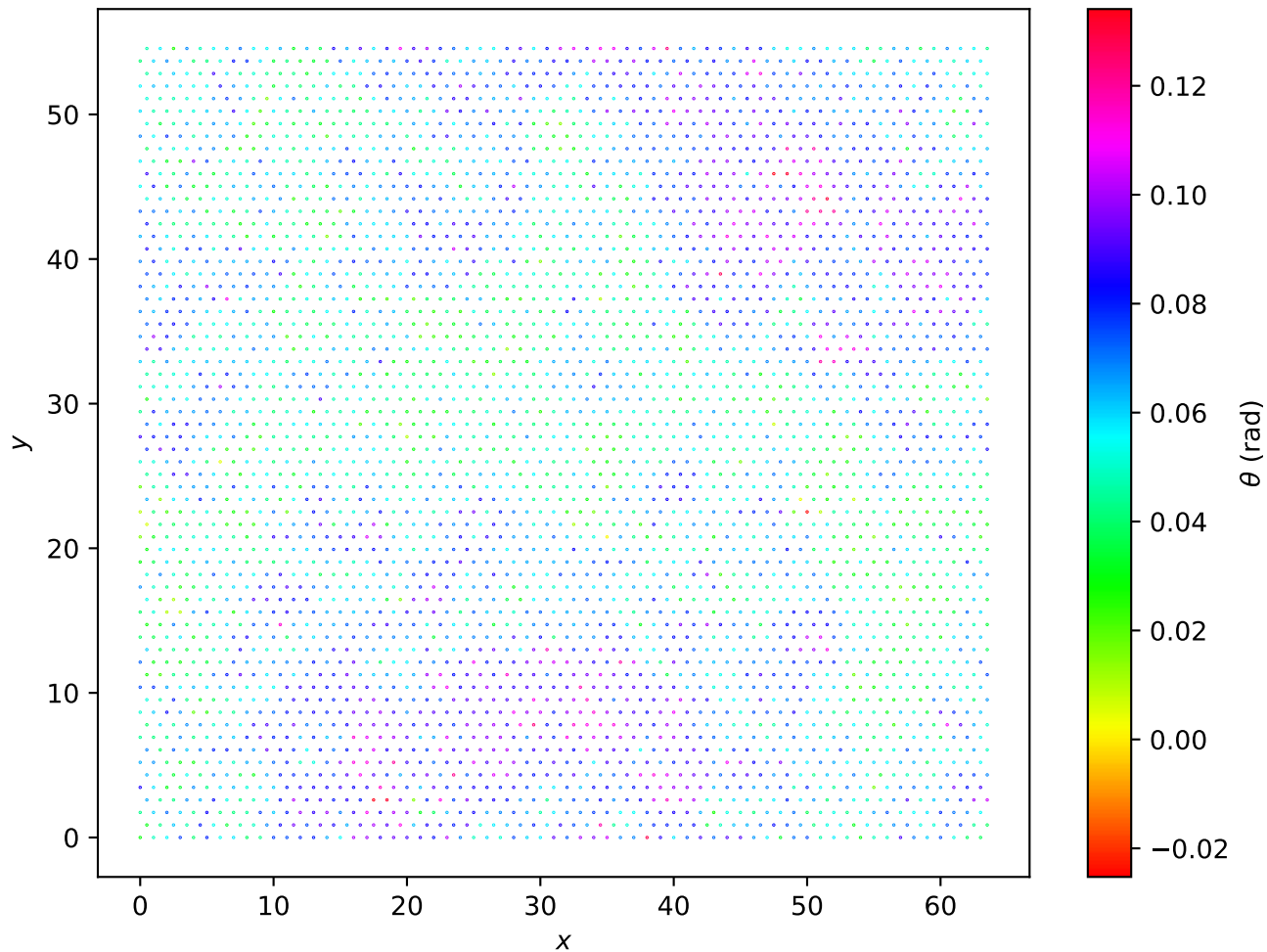
Hexagonal Lattice L=64 , T = 5.00e - 02
