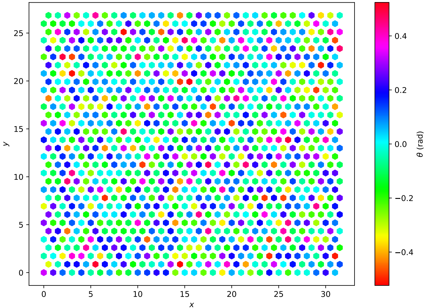
Hexagonal Lattice L=32 , T = 1.00e - 01
