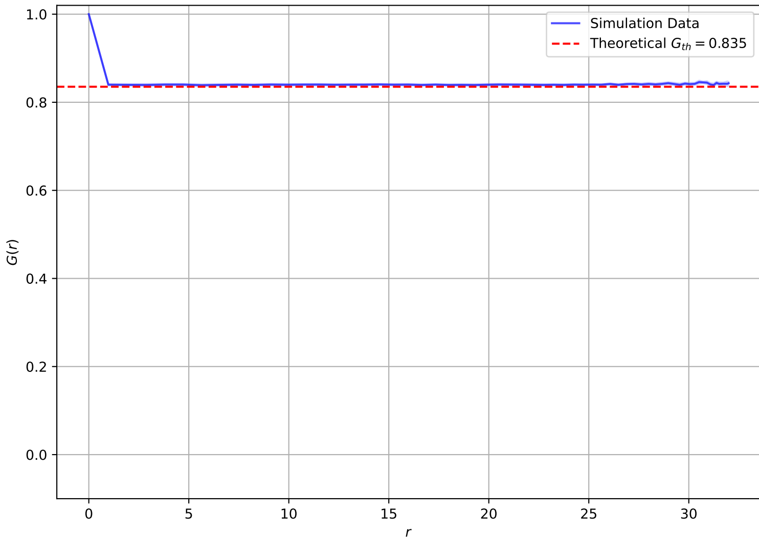
Correlation Function at T = 1.00\text{e} - 02 , L = 32
