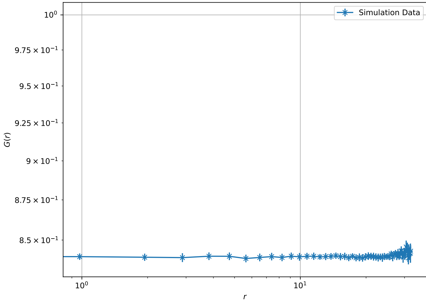
Correlation Function at T = 1.00\text{e} - 02 , L = 32 (Log-Log Scale)
