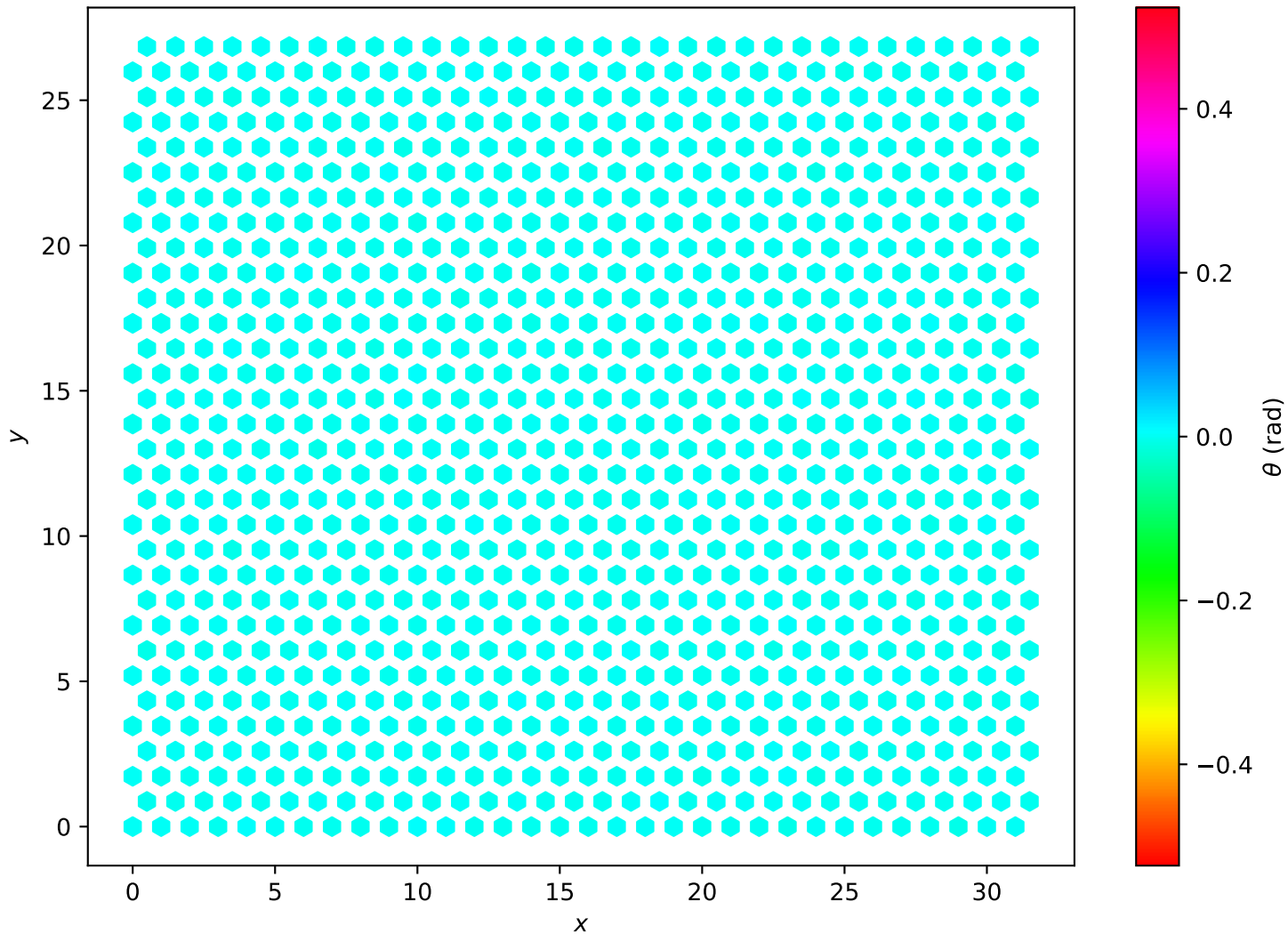
Hexagonal Lattice L=32 , T = 1.00e - 05
