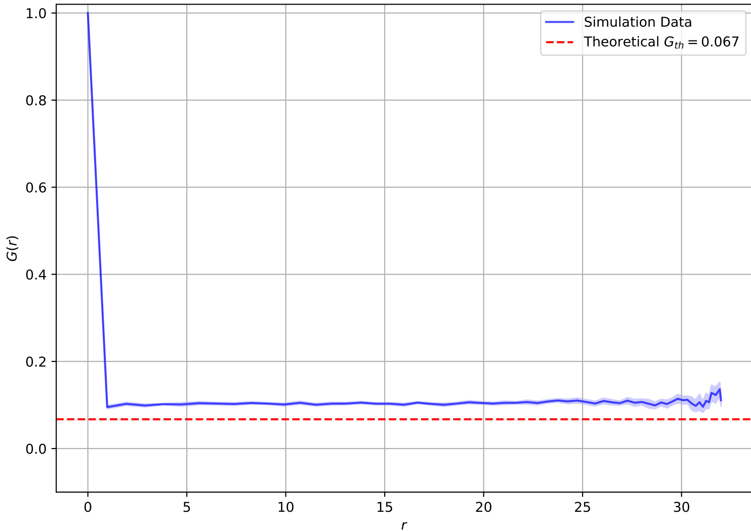
Correlation Function at T = 1.50e - 01 , L = 32
