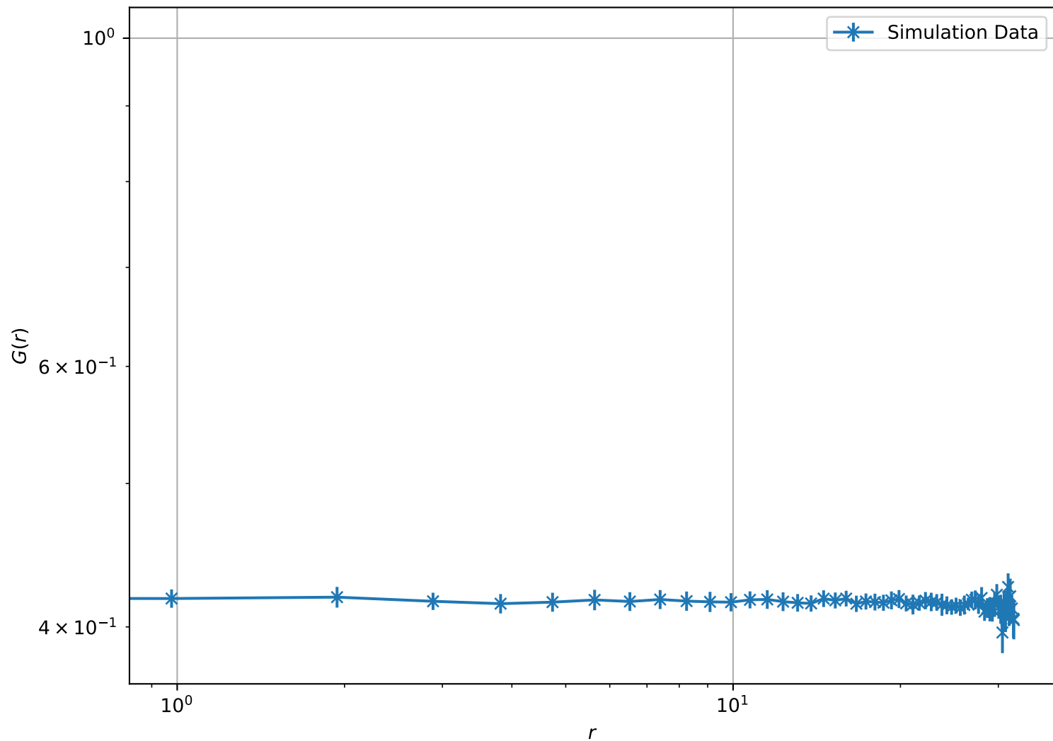
Correlation Function at T = 5.00\text{e} - 02 , L = 32 (Log-Log Scale)
