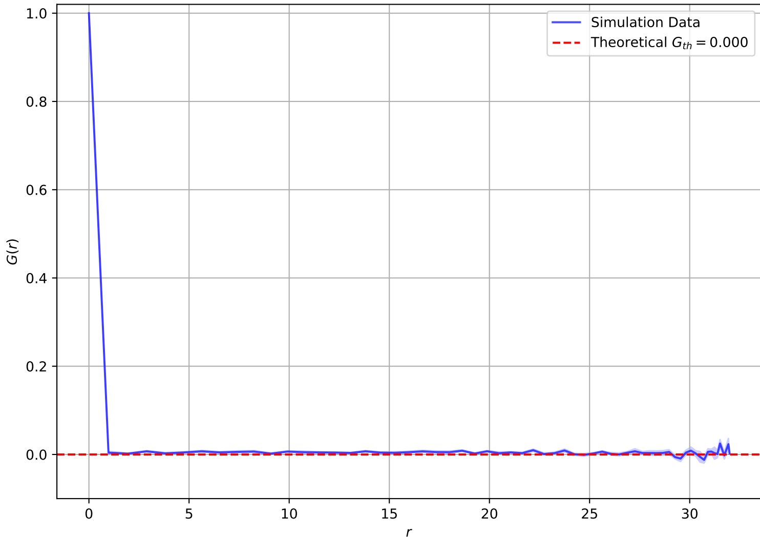
Correlation Function at T = 8.00e - 01 , L = 32
