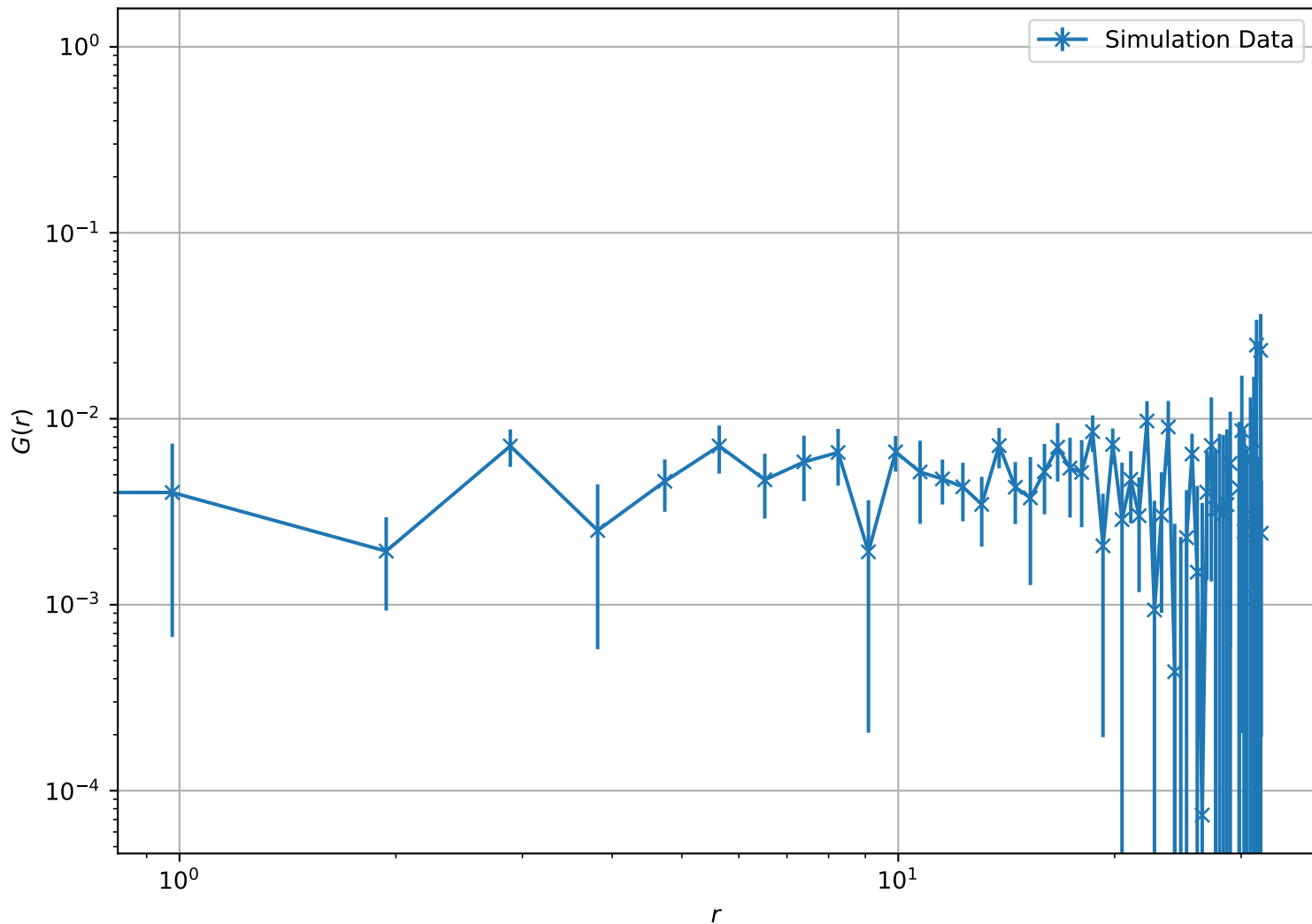
Correlation Function at T = 8.00\text{e} - 01 , L = 32 (Log-Log Scale)
