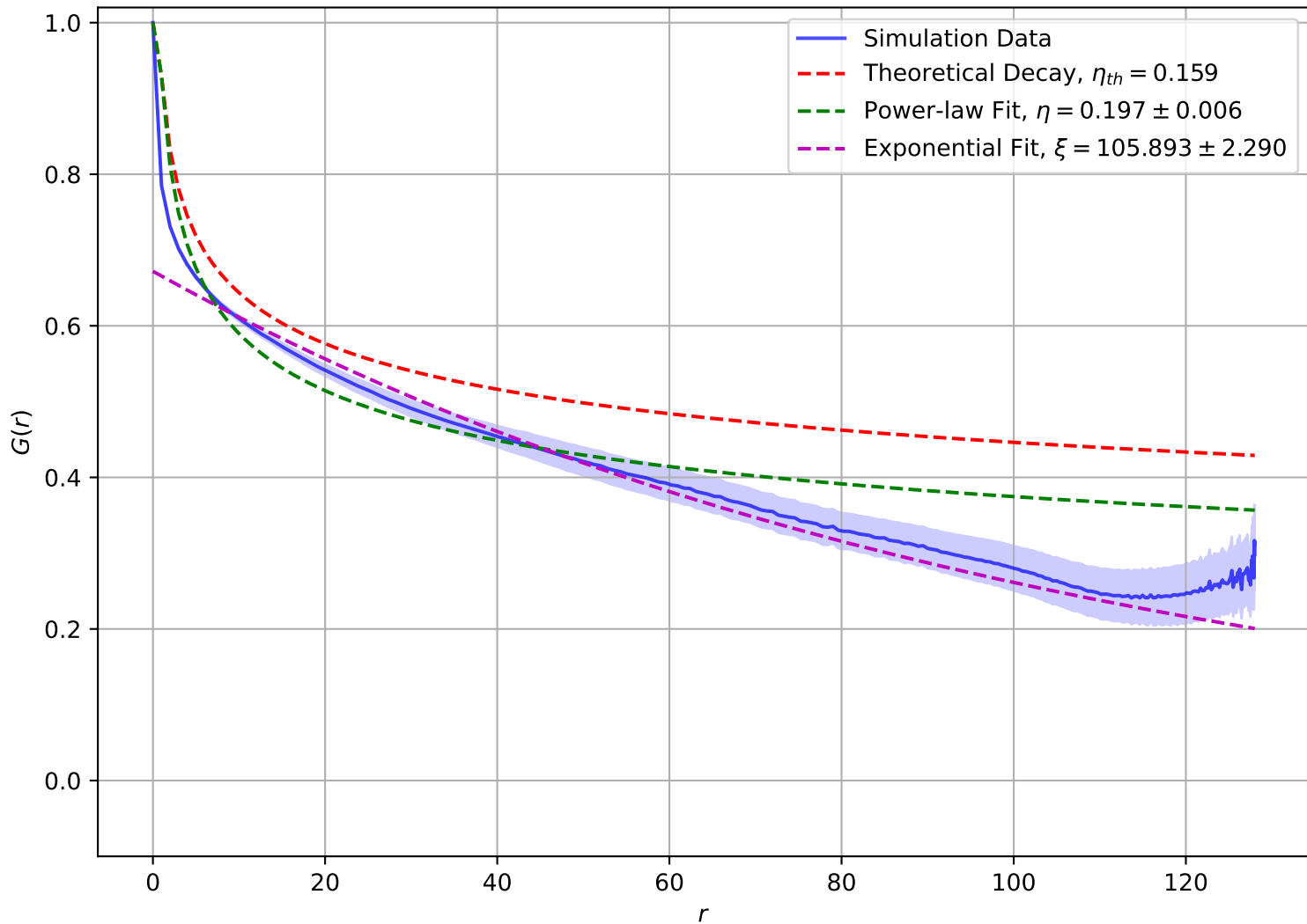
Correlation Function at T = 1.00e + 00 , L = 128
