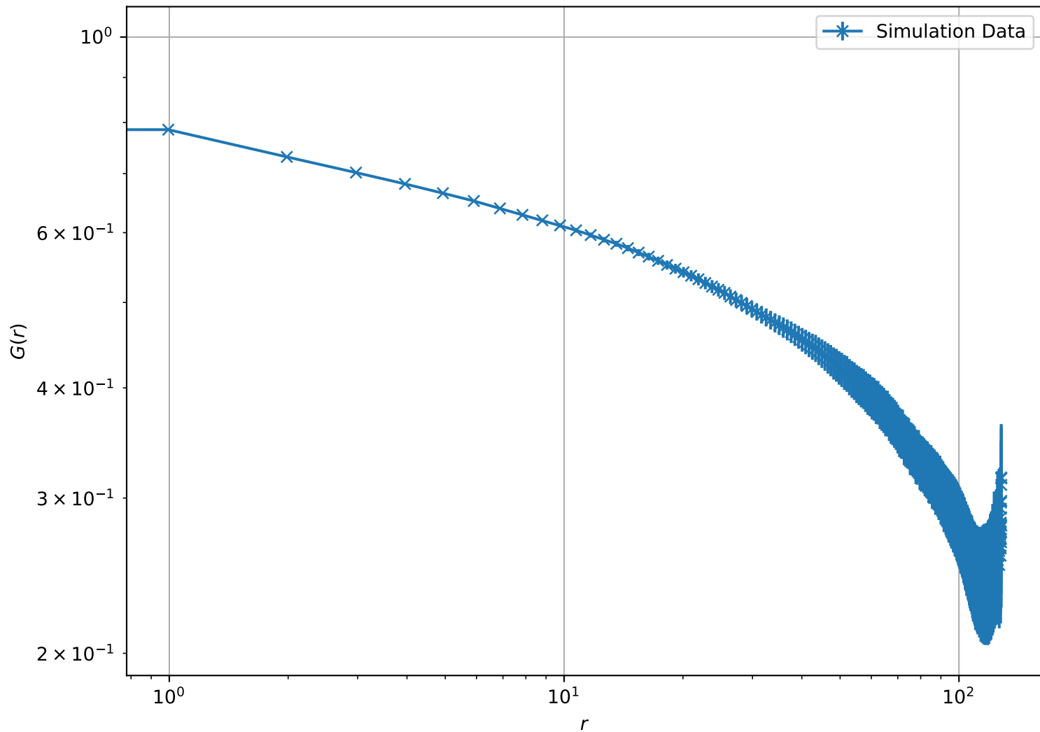
Correlation Function at T = 1.00e + 00 , L = 128 (Log-Log Scale)
