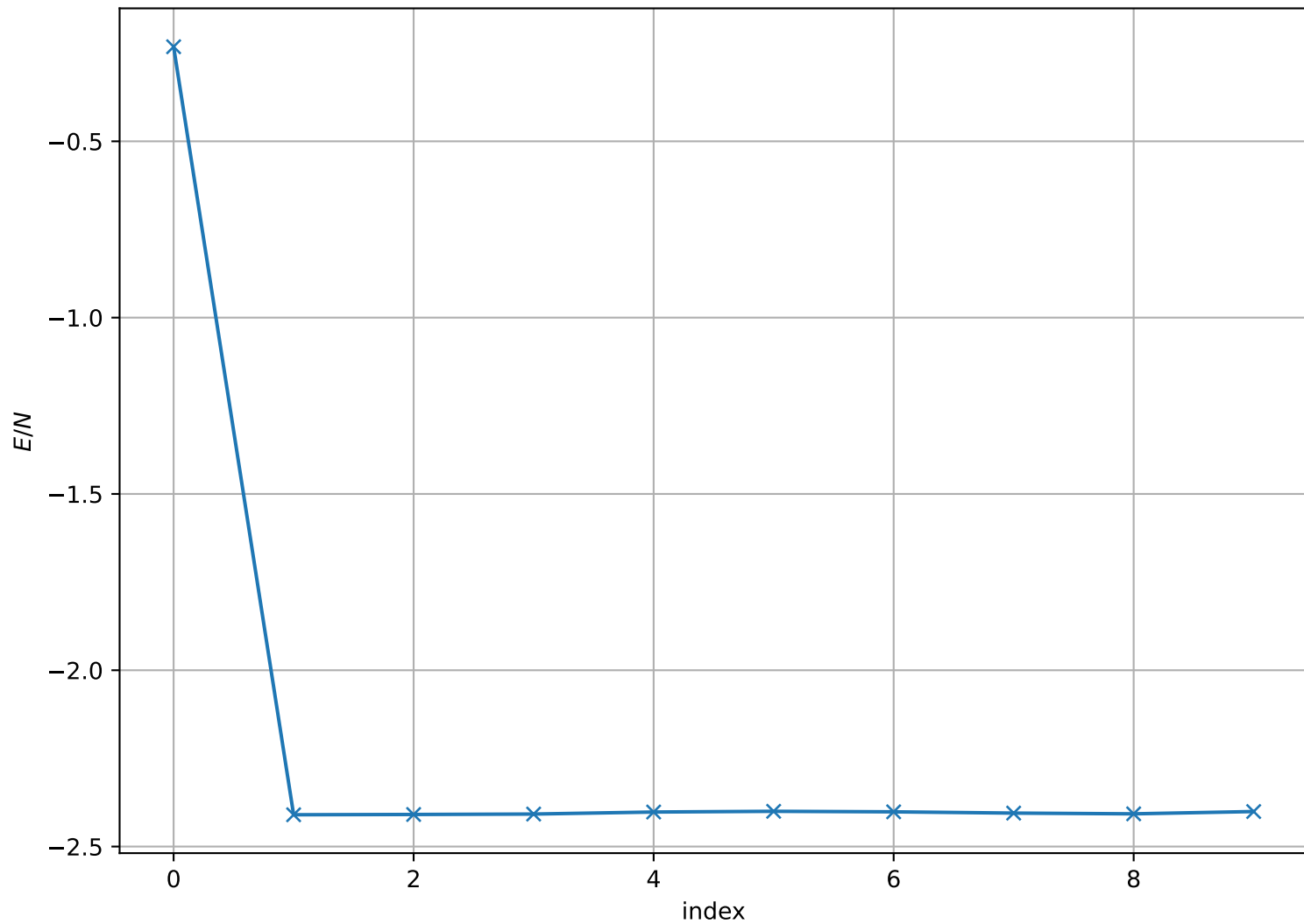
Energy per Site at T = 1.000e + 00 , L = 128
