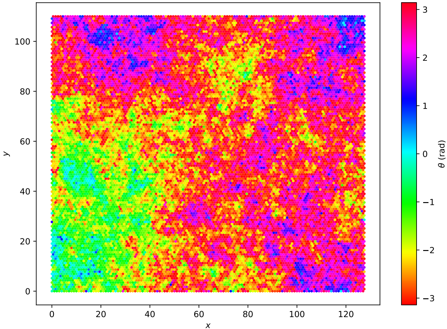
Hexagonal Lattice L=128 , T = 1.00e + 00
